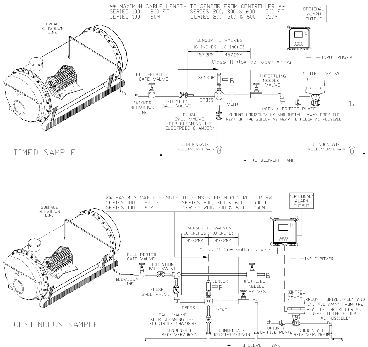
FIGURE 1 Typical Installation
