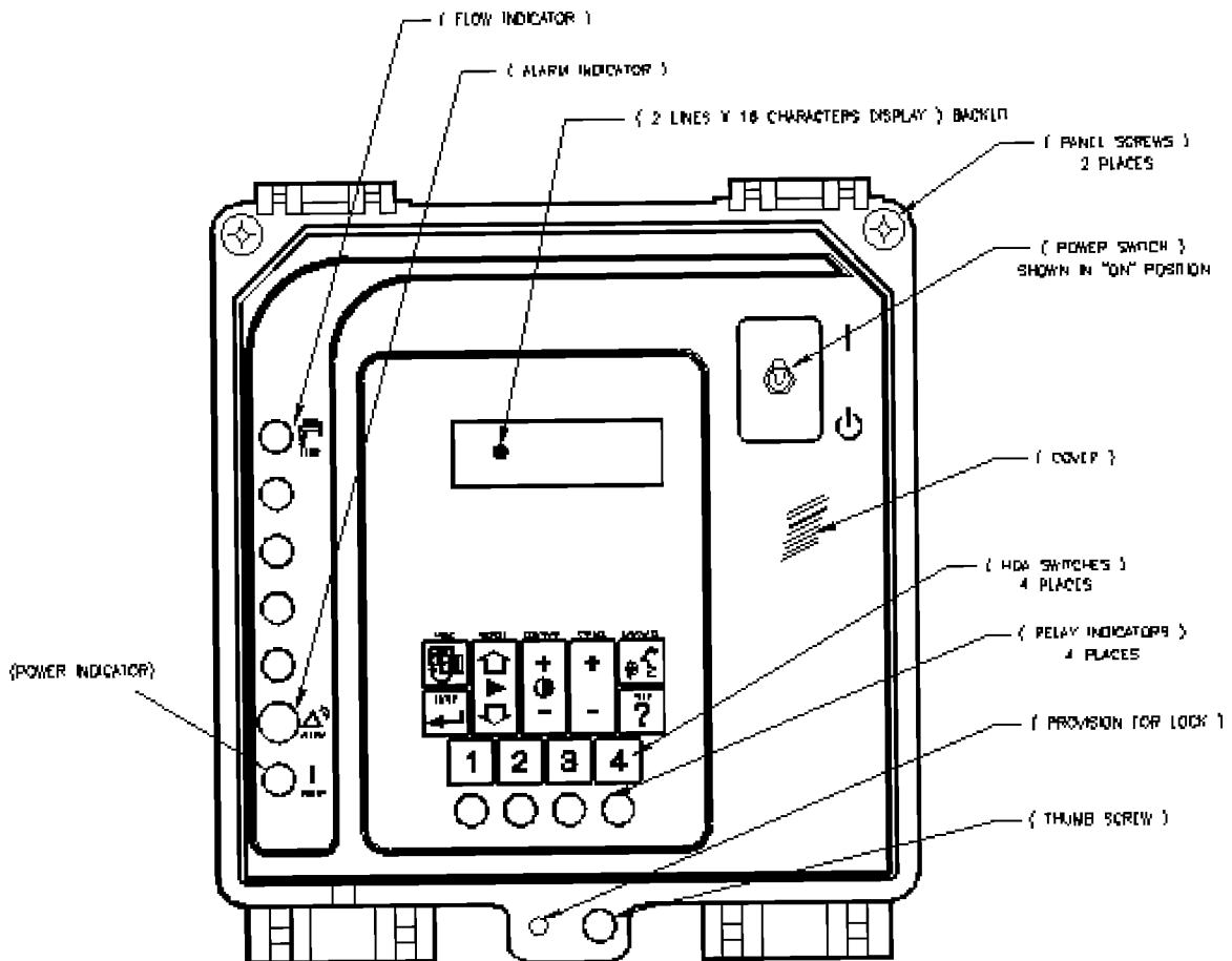
FIGURE 2 9200 Series Front Panel
