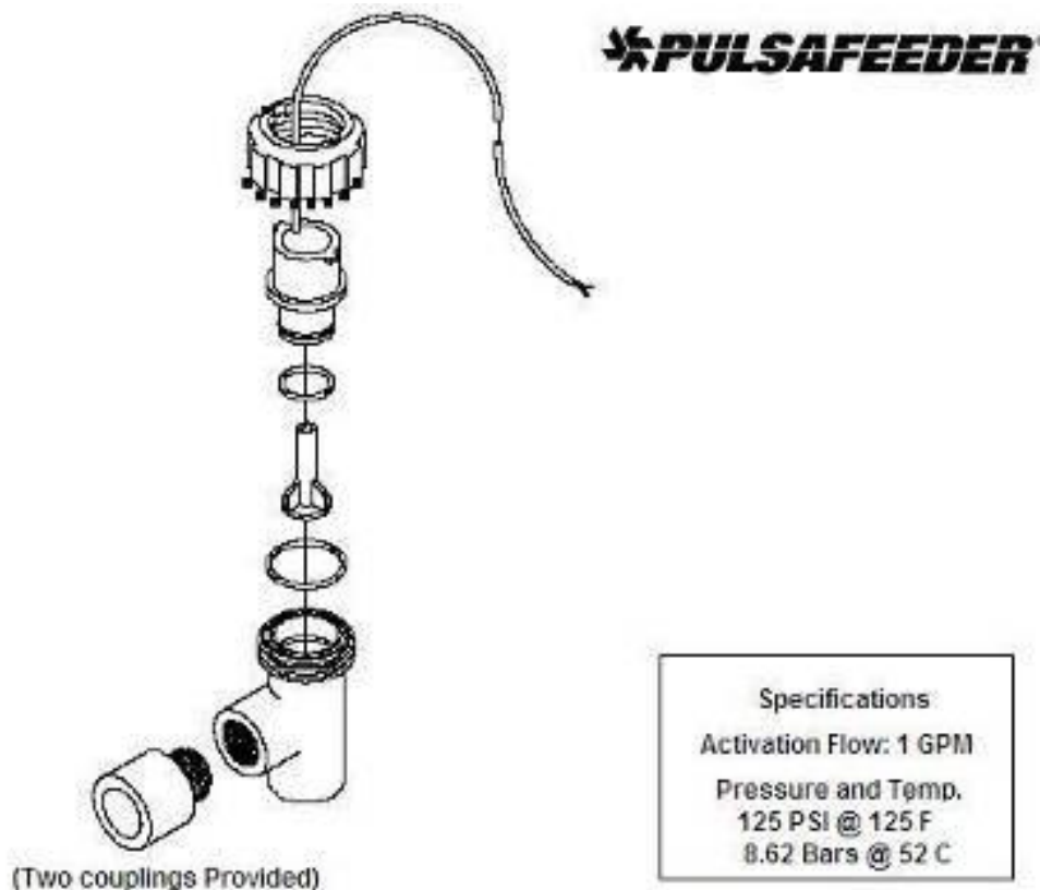
P/N 04-350-90-1 Flow Switch Assembly
