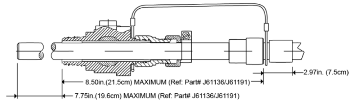
MODEL #J61136 / J61191
