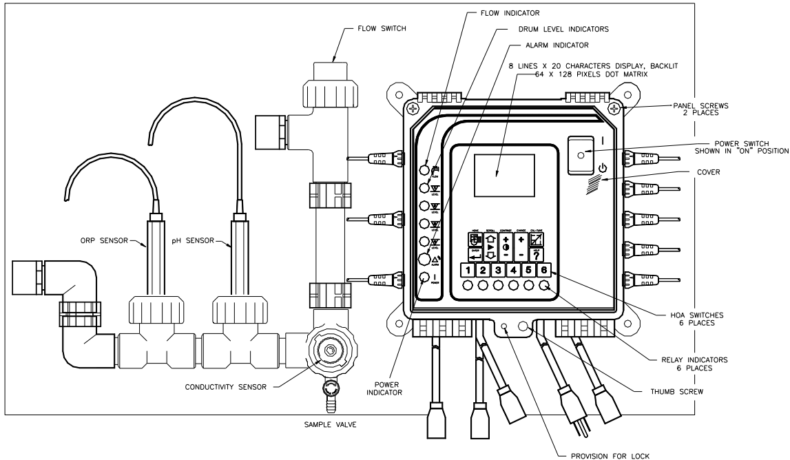
Figure 4 – Front Panel
