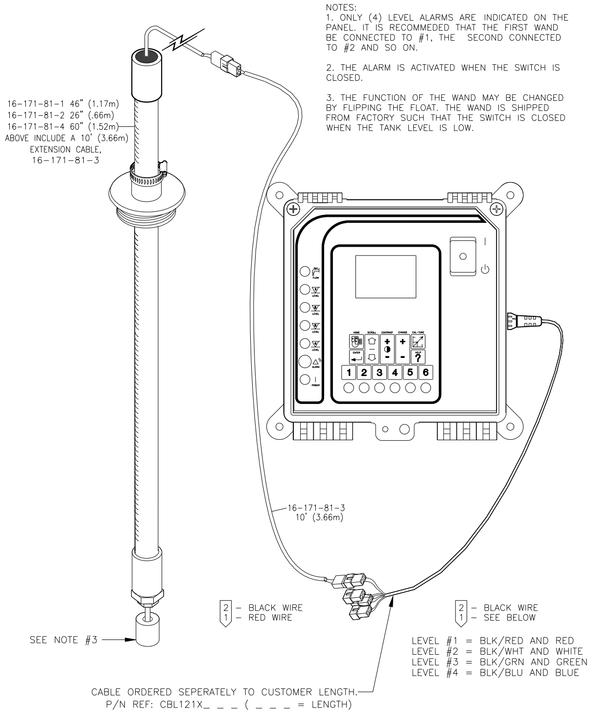
DIAGRAM 11 – SINGLE POINT DRUM LEVEL WAND
