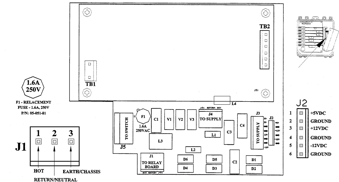
DIAGRAM 10 – POWER SUPPLY STANDARD / CE
