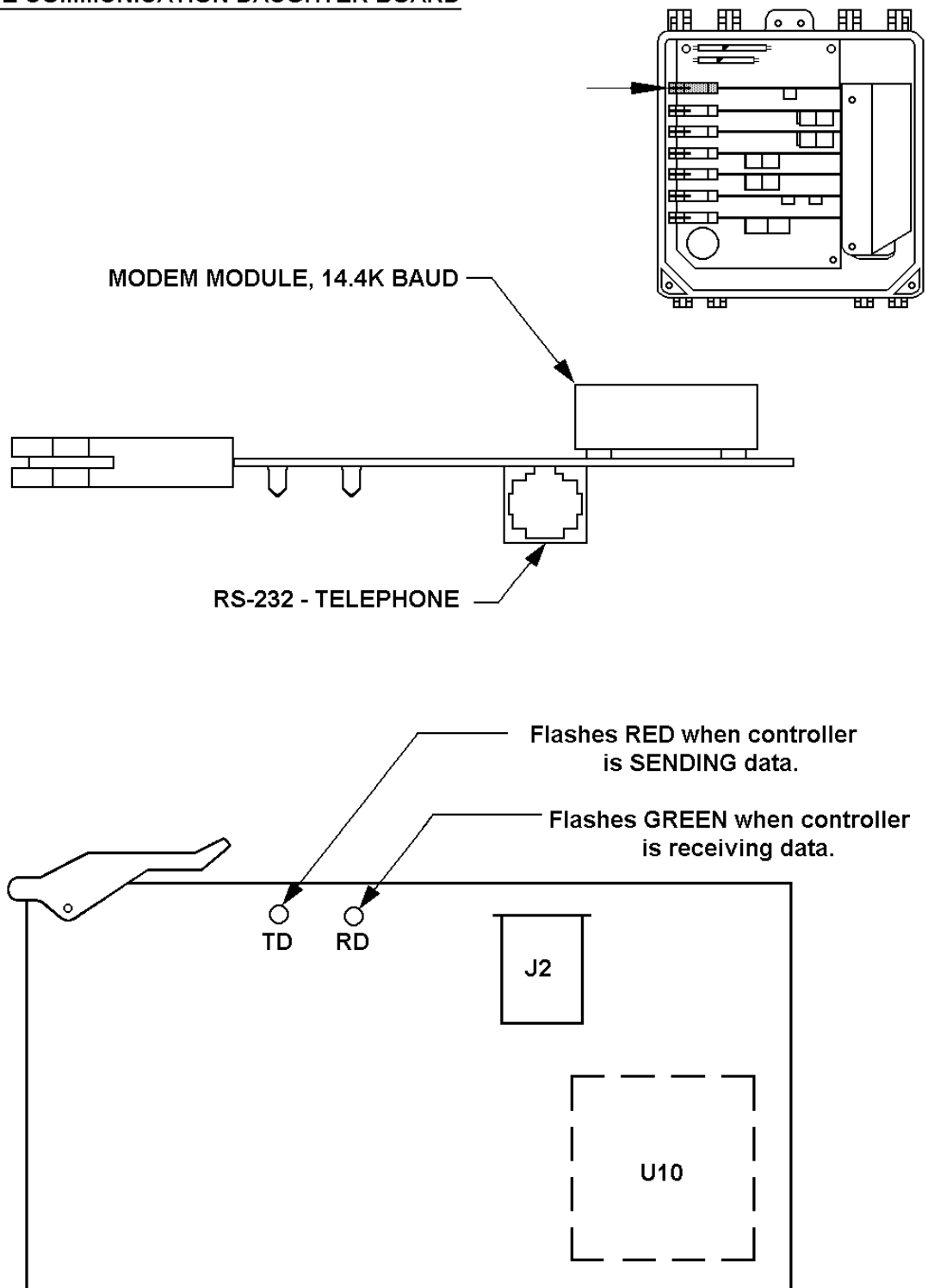
DIAGRAM 9A – SERIAL / INTERNAL MODEM COMMUNICATIONS DAUGHTER BOARD
