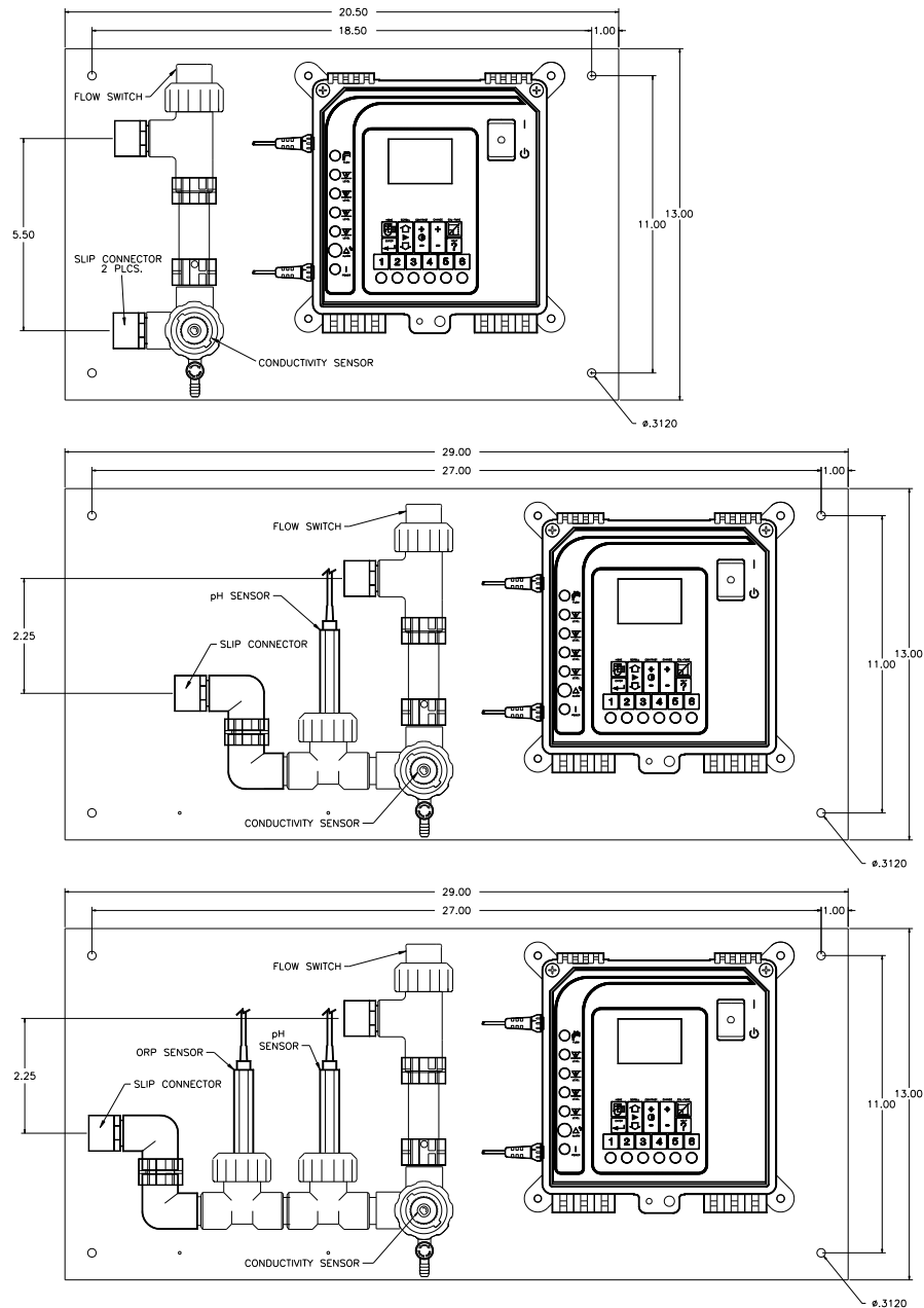
DIAGRAM 1 – ENCLOSURE DIMENSIONAL DATA
