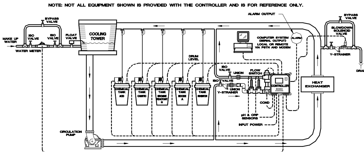
Figure 1 – Typical Installation
