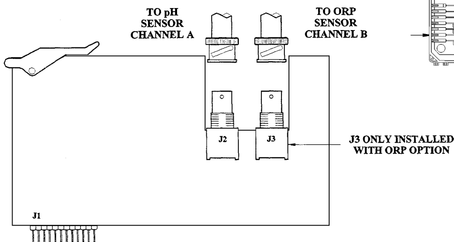
DIAGRAM 5 CONDUCTIVITY / pH / ORP DAUGHTER BOARD
